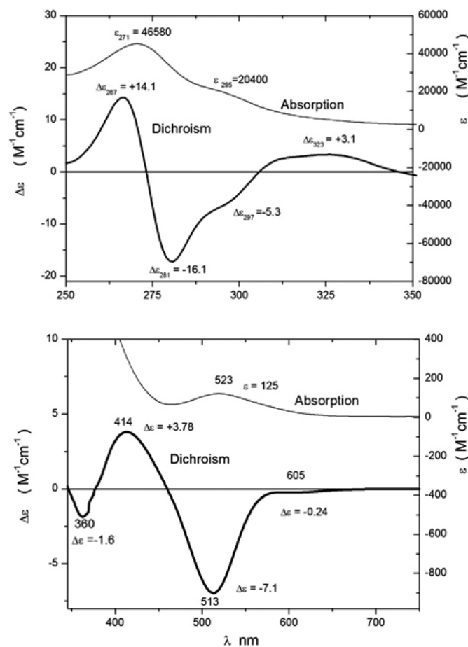
Figure 1: Absorption and circular dichroism (CD) spectra of [\text{Co}(\text{phen})_2\text{lactose}]^{2+} complex (1).
