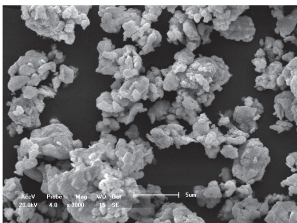
Figure 2. SEM \text{Co}_{87}\text{Nb}_{46}\text{B}_{15} amorphous alloy forming irregular grains.
