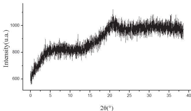
Figure 1. Spectrum of XRD amorphous alloy \text{Co}_{87}\text{Nb}_{46}\text{B}_{15} .
