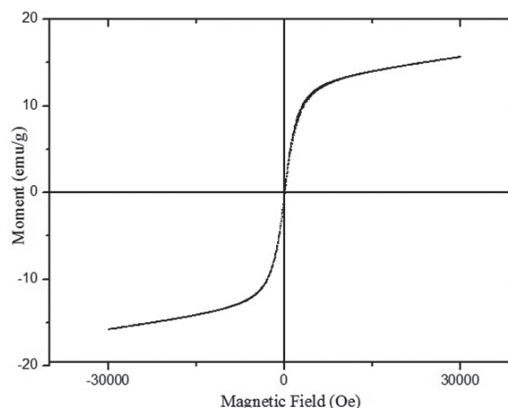
Figure 4. Hysteresis curve of amorphous alloy \text{Co}_{87}\text{Nb}_{46}\text{B}_{15} .
