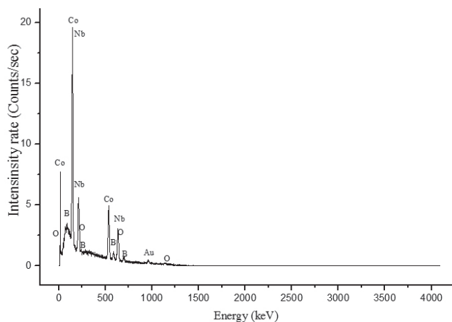
Figure 3. Analysis of EDS amorphous alloy \text{Co}_{87}\text{Nb}_{46}\text{B}_{15} .
